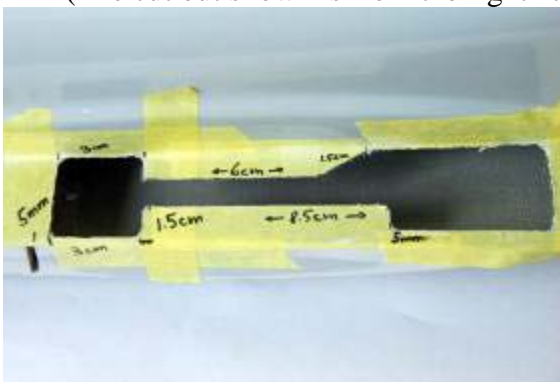
Mask the remaining area as shown above and in the template. (The cut out shown is from the right hand side of the model viewed from below)
